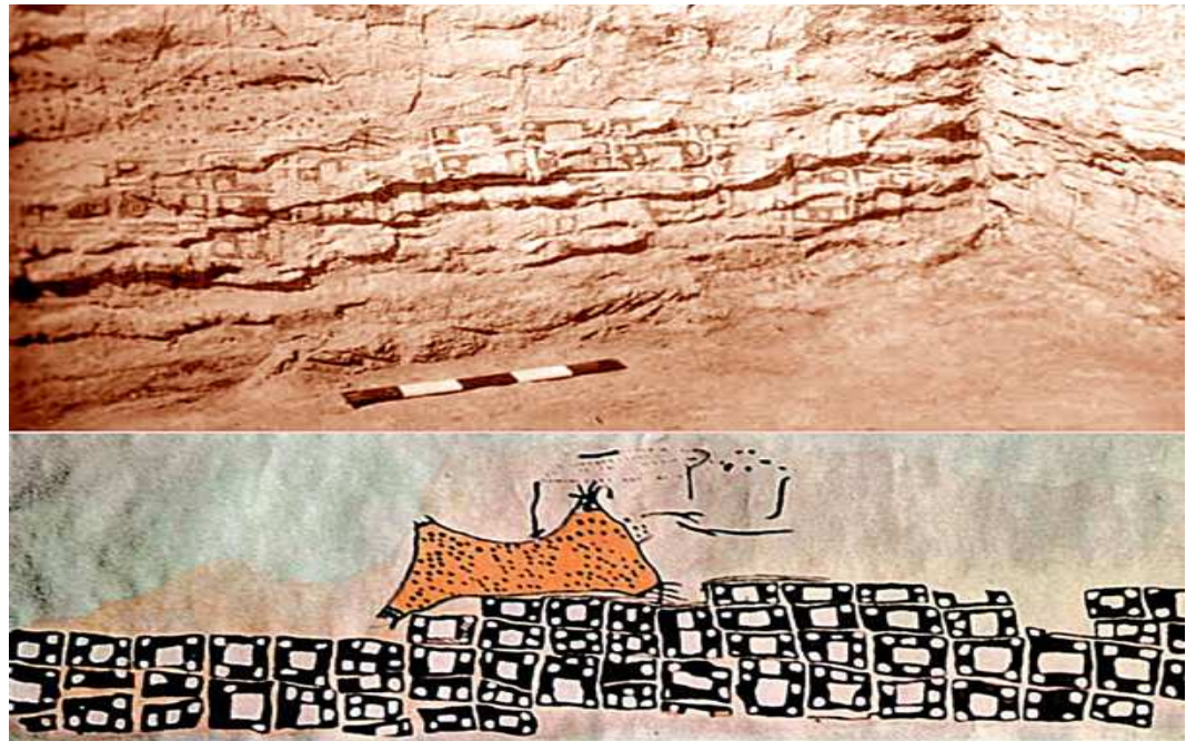
Fig. 2 - a) Wall graffiti b) painting interpreted as a bird's eye view of the megalithic village of Çatalhöyük in Turkey.
